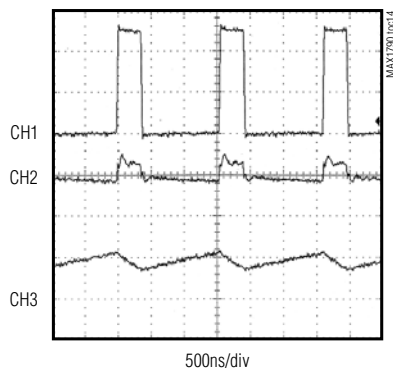
SWITCHING WAVEFORM
