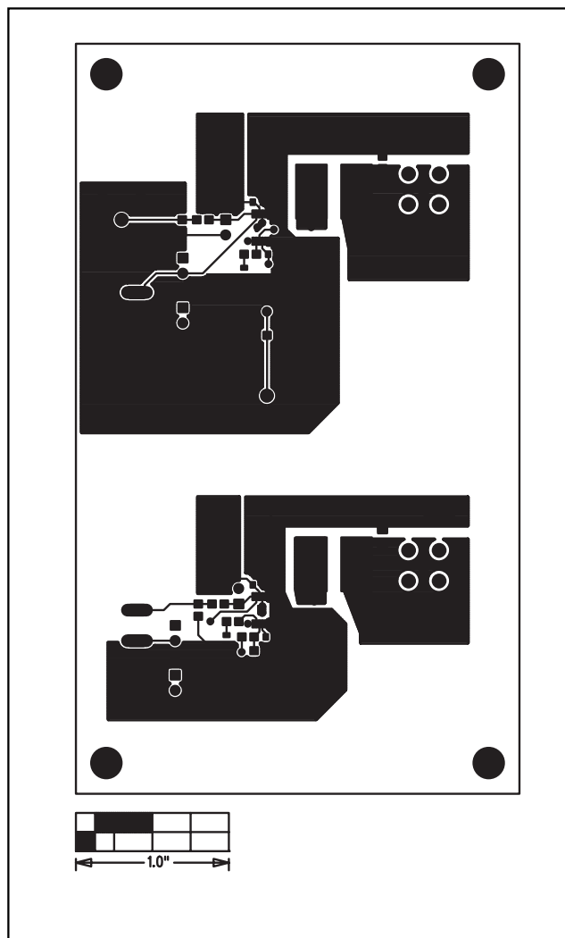
Figure 4. MAX1820 EV Kit PC Board Layout—Component Side
