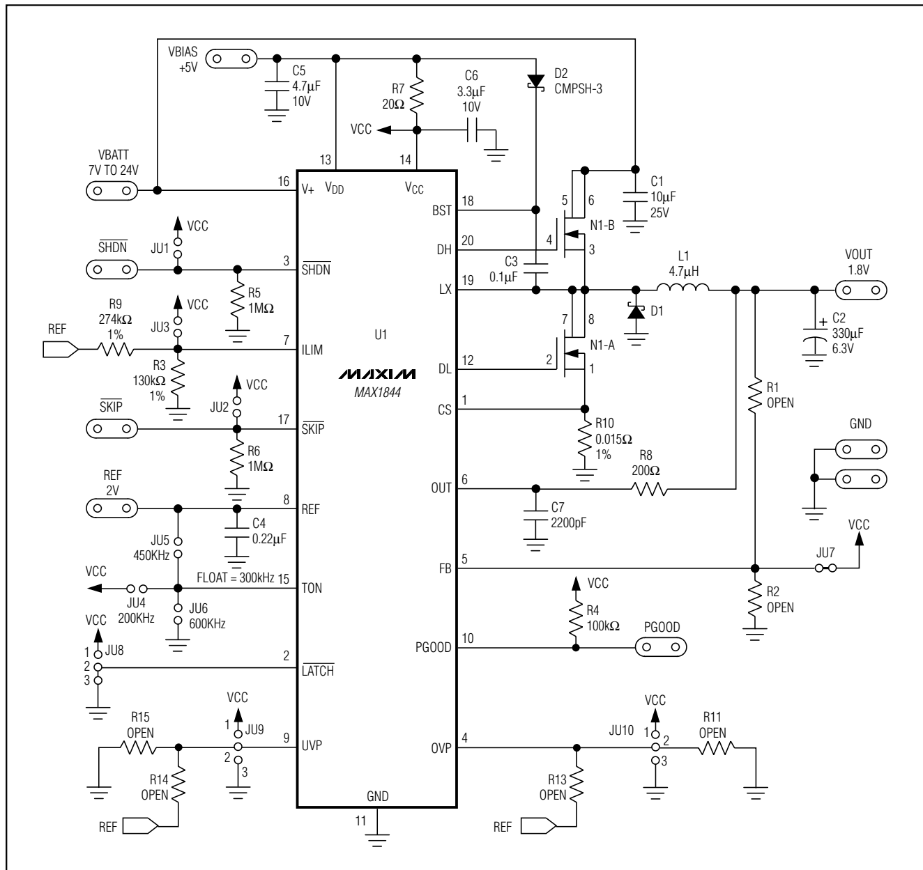
Figure 1. MAX1844 EV Kit Schematic
