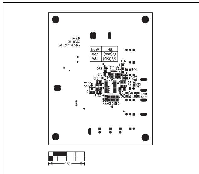
Figure 7. MAX1845 EV Kit Component Placement Guide—Solder Side
