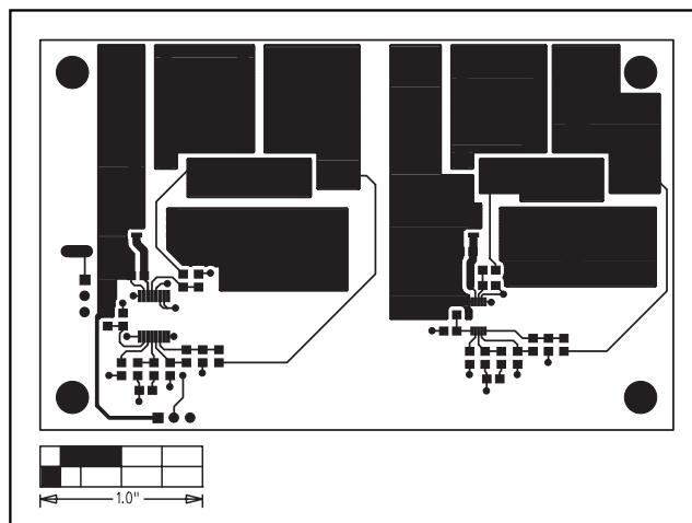
Figure 4. MAX1846 EV Kit PC Board Layout—Component Side
