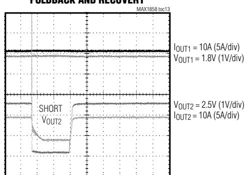
SHORT-CIRCUIT CURRENT FOLDBACK AND RECOVERY
