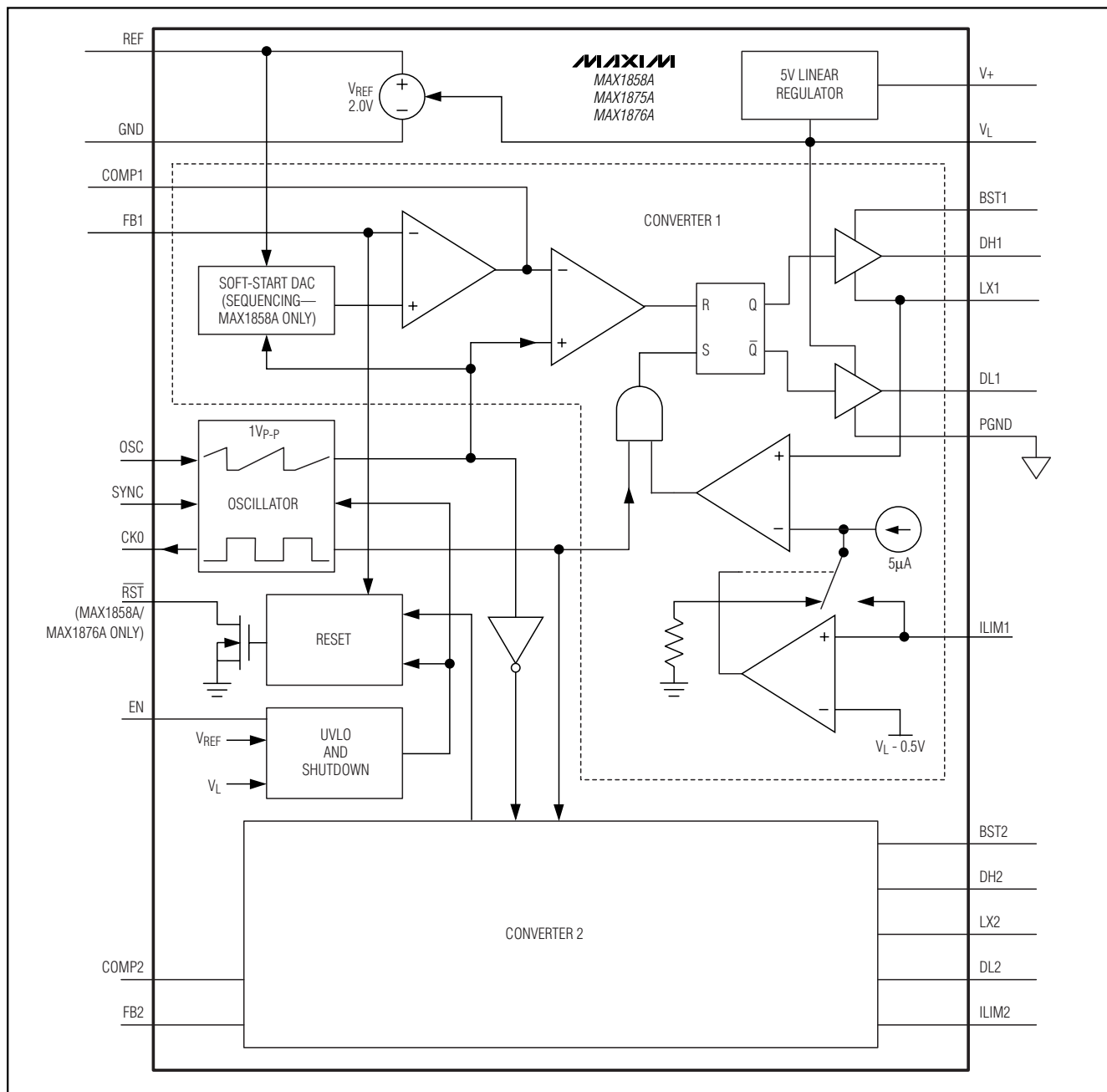
Figure 2. Functional Diagram
