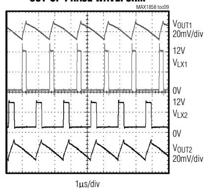
OUT-OF-PHASE WAVEFORM
