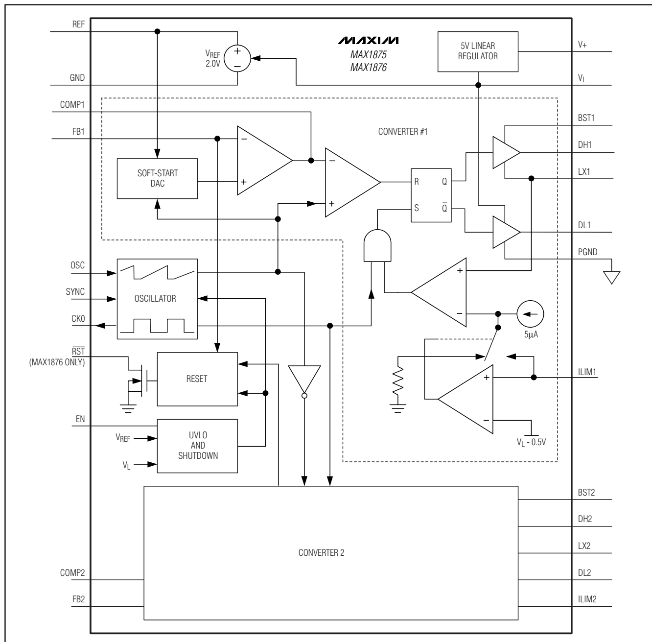
Figure 2. Functional Diagram
