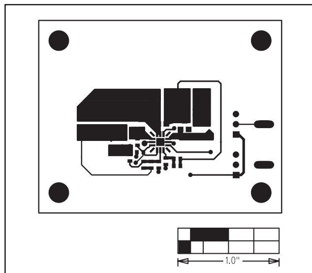
Figure 3. MAX1878 EV Kit PC Board Layout—Component Side
