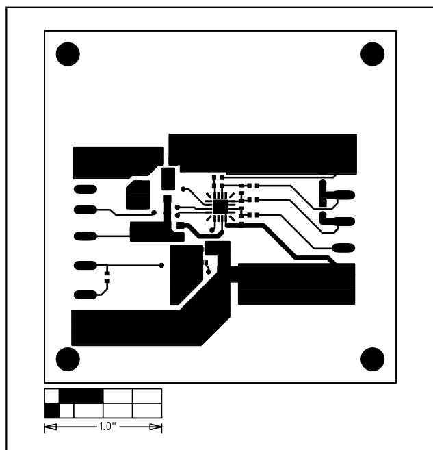
Figure 3. MAX1906 EV Kit PC Board Layout—Component Side
