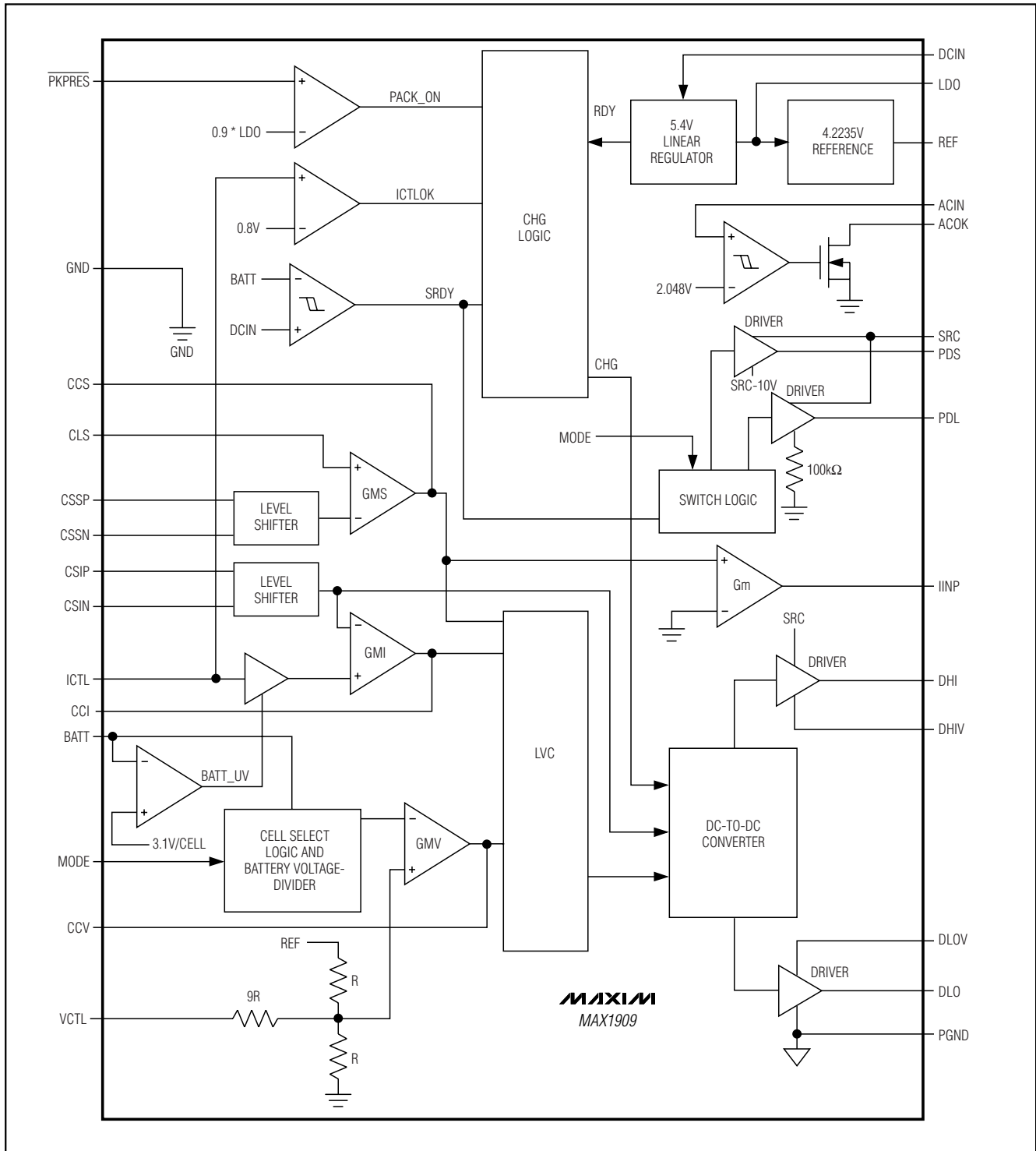
Figure 3. Functional Diagram
