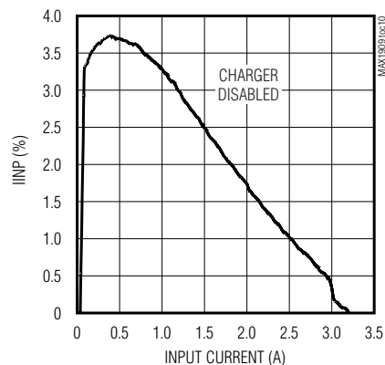
IINP ERROR vs. INPUT CURRENT
