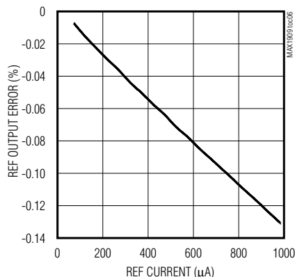
REF LOAD REGULATION
