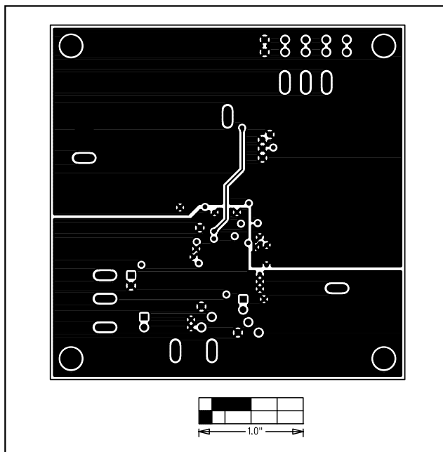
Figure 5. MAX1909 EV Kit PC Board Layout—Ground Layer
