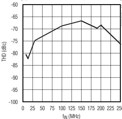
THD vs. ANALOG INPUT FREQUENCY ( f_{SAMPLE} = 170.0043MHz , A_{IN} = -1dBFS )
