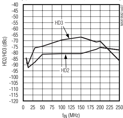
HD2/HD3 vs. ANALOG INPUT FREQUENCY ( f_{SAMPLE} = 170.0043MHz , A_{IN} = -1dBFS )
