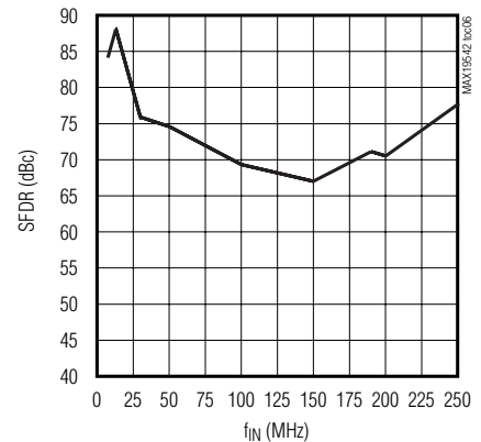
SFDR vs. ANALOG INPUT FREQUENCY ( f_{SAMPLE} = 170.0043MHz , A_{IN} = -1dBFS )
