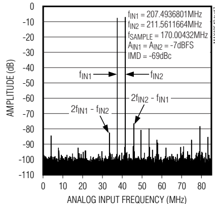
TWO-TONE IMD (16,384-POINT DATA RECORD)
