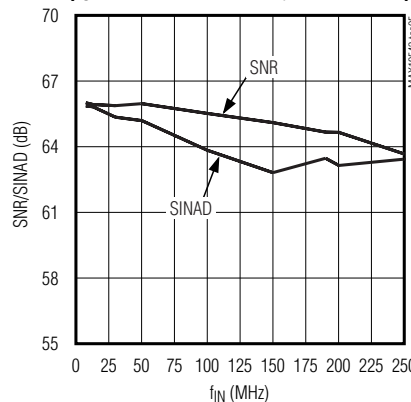
SNR/SINAD vs. ANALOG INPUT FREQUENCY ( f_{SAMPLE} = 170.0043MHz , A_{IN} = -1dBFS )
