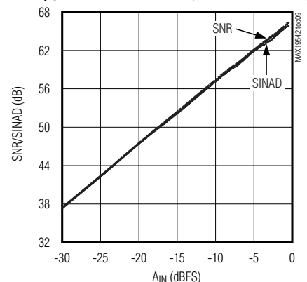
SNR/SINAD vs. ANALOG INPUT AMPLITUDE ( f_{SAMPLE} = 170.0043MHz , f_{IN} = 64.9864MHz )
