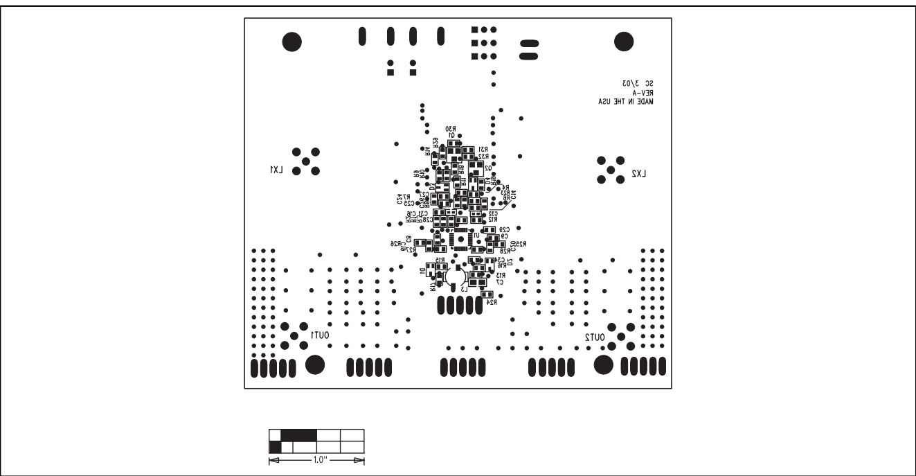
Figure 3. MAX1955 EV Kit Component Placement Guide—Solder Side
