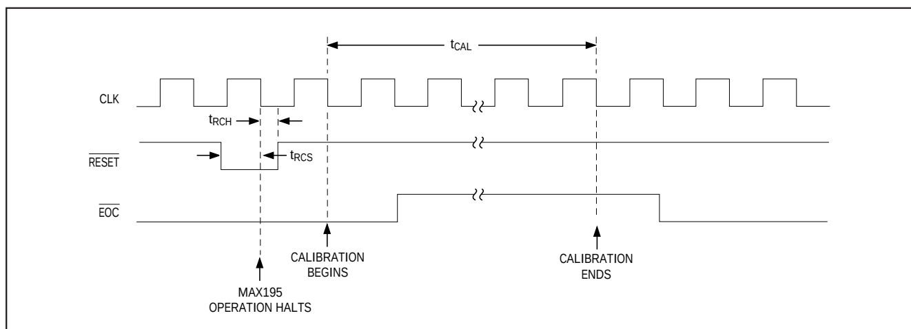
Figure 2. Initiating Calibration
