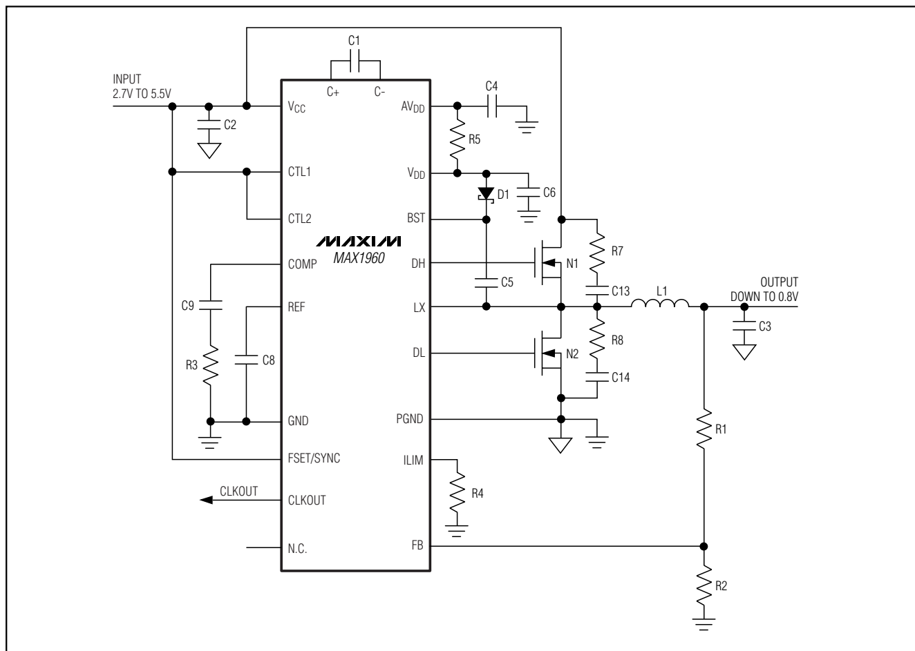
Figure 9. Application Circuit 1—MAX1960 Adjustable Output Voltage
