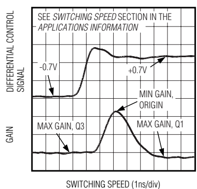
SWITCHING SPEED
