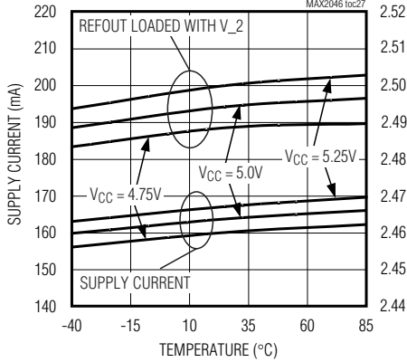
REFOUT AND SUPPLY CURRENT vs. TEMPERATURE AND SUPPLY VOLTAGE
