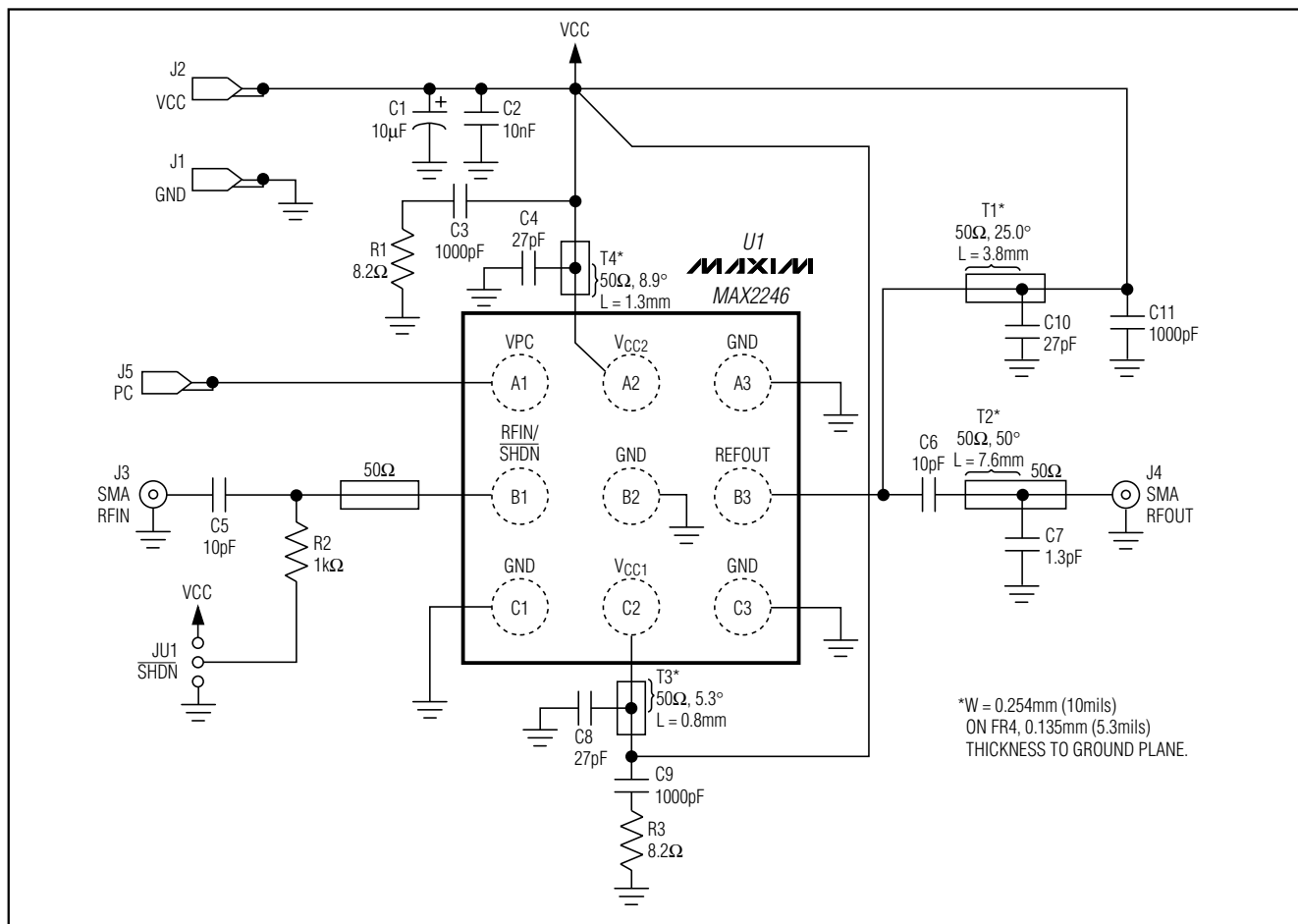
Figure 2. MAX2246 EV Kit Schematic
