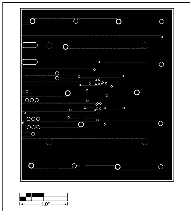
Figure 3. MAX2700/MAX2701 EV Kits PC Board Layout—Ground Plane
