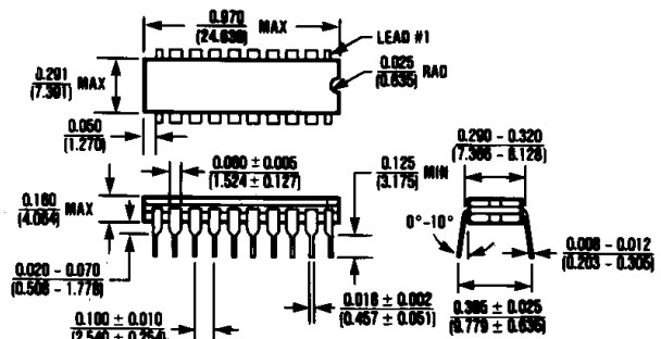
20 Lead Cerdip
