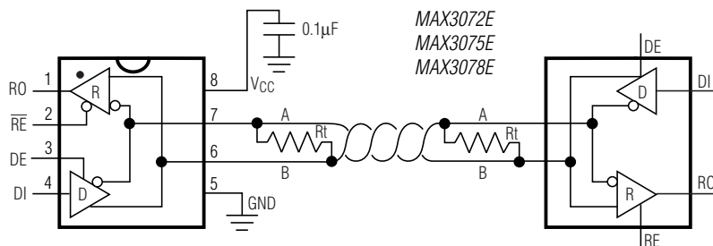
TYPICAL HALF-DUPLEX OPERATING CIRCUIT
