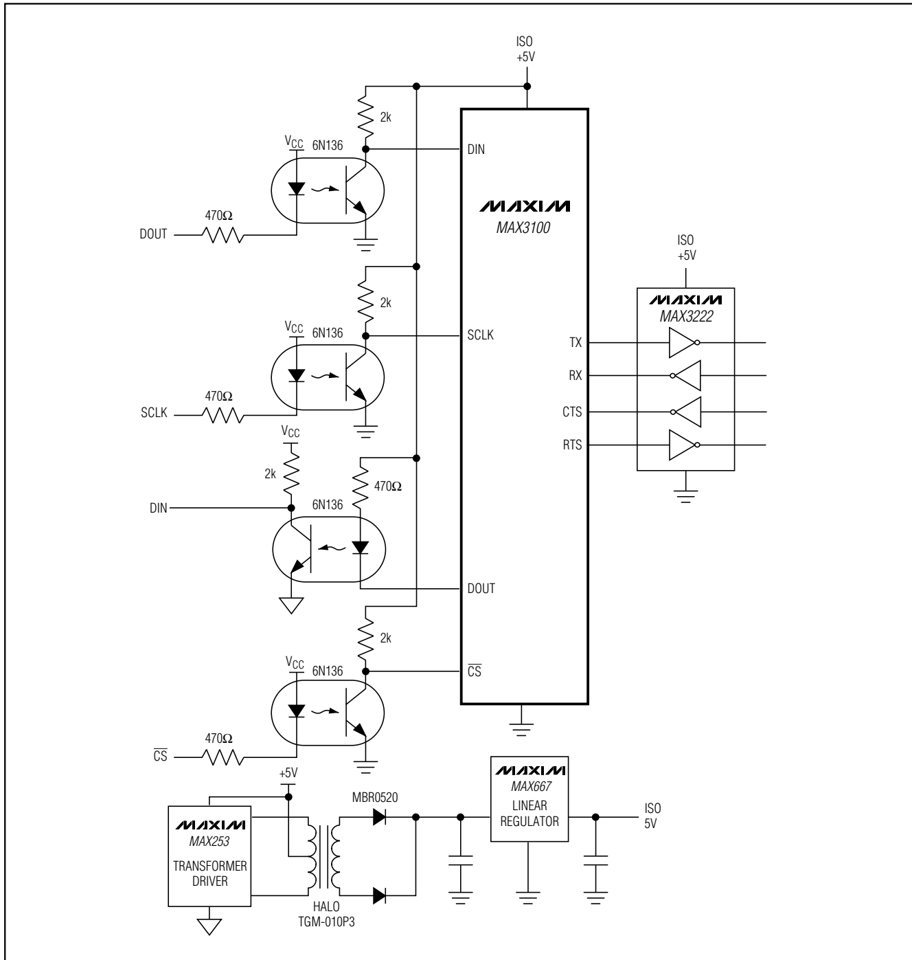
Figure 7. Driving Optocouplers
