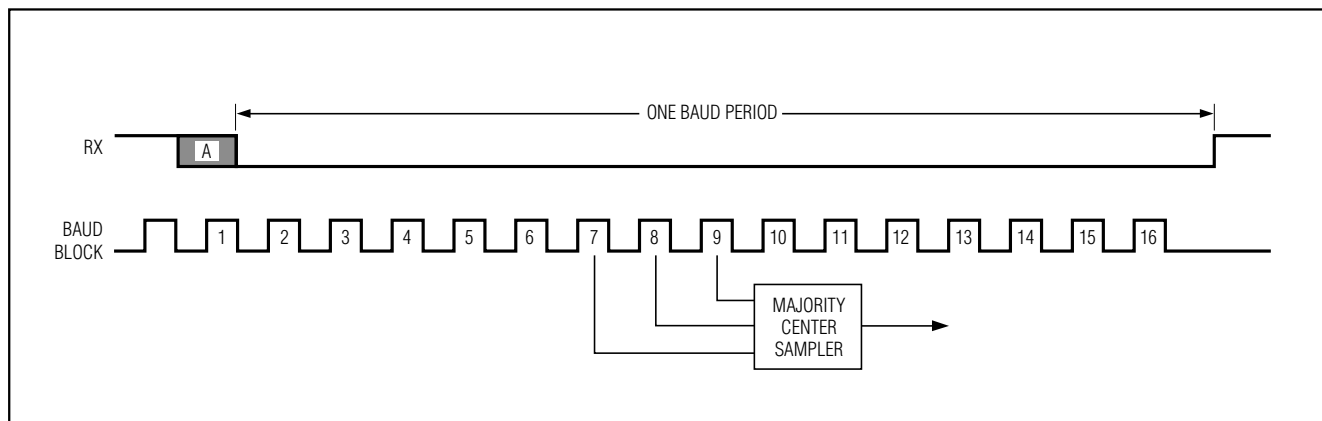
Figure 3. Start-Bit Timing
