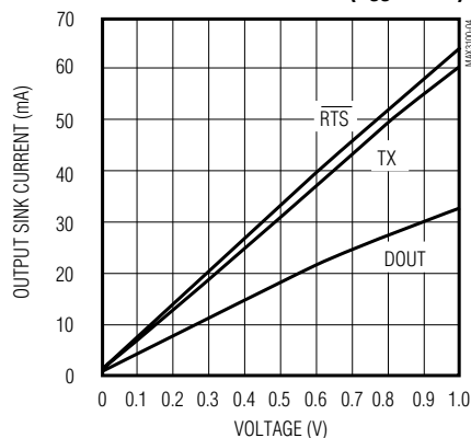
TX, \overline{\text{RTS}} , DOUT OUTPUT CURRENT vs. OUTPUT LOW VOLTAGE ( V_{CC} = 3.3V )
