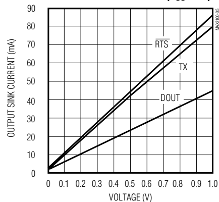
TX, \overline{\text{RTS}} , DOUT OUTPUT CURRENT vs. OUTPUT LOW VOLTAGE ( V_{CC} = 5V )
