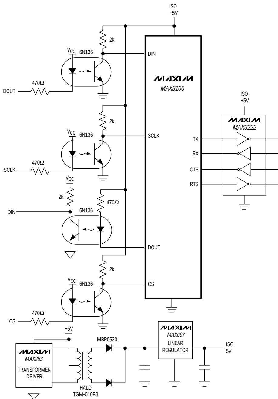
Figure 7. Driving Optocouplers
