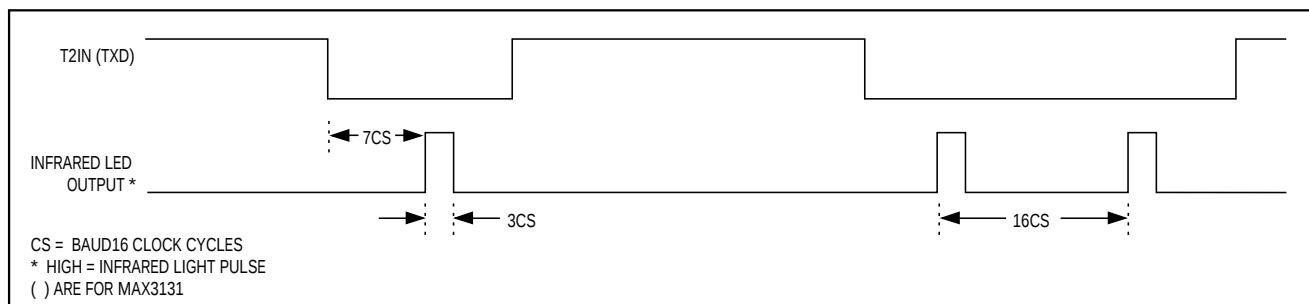
Figure 3b. ENDEC Operation, Transmitting Infrared
