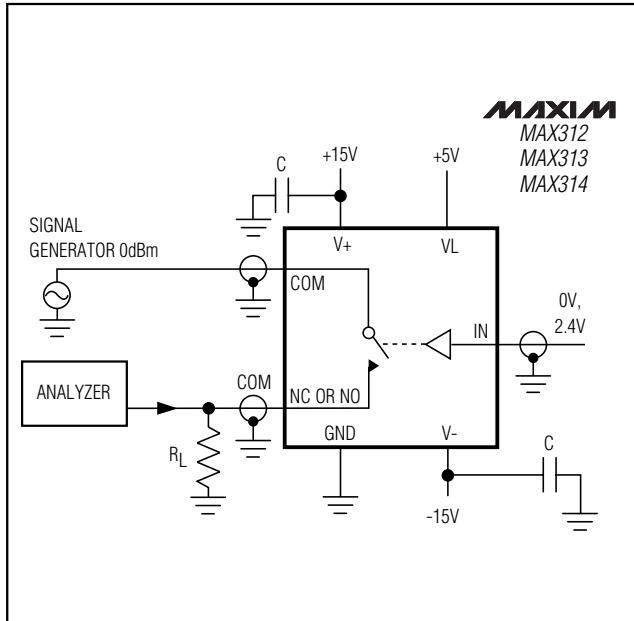
Figure 5. Off-Isolation Test Circuit
