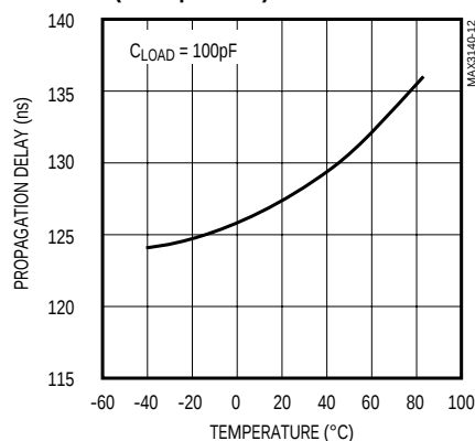
RS-485 DRIVER PROPAGATION DELAY (500kbps MODE) vs. TEMPERATURE
