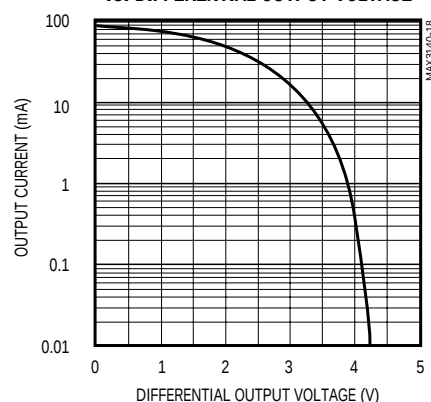
RS-485 DRIVER OUTPUT CURRENT vs. DIFFERENTIAL OUTPUT VOLTAGE
