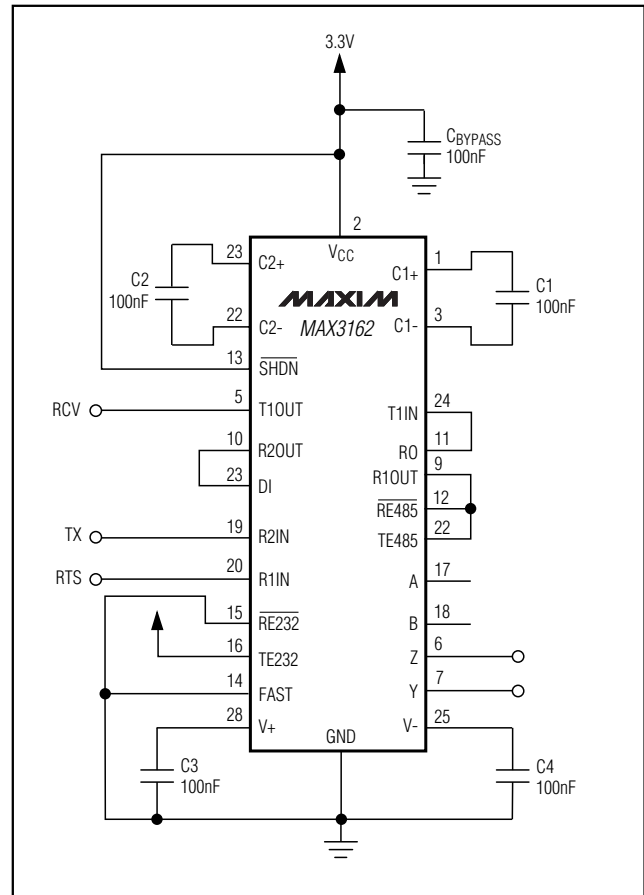
Figure 15. Protocol Translator
