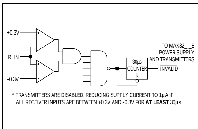
Figure 3a. MAX32__E Entering 1\mu\text{A} Supply Mode via AutoShutdown
