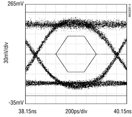
MAX3261CCJ EYE DIAGRAM (622Mbps, LOAD AT OUT- = 1300nm LASER WITH 467MHz BESSEL FILTER)*
