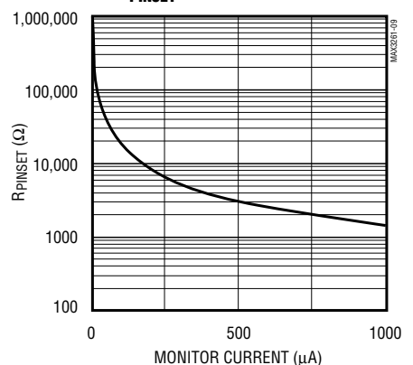
RPINSET VS. MONITOR CURRENT
