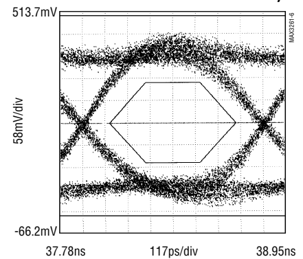
MAX3261CCJ EYE DIAGRAM (1062Mbps, LOAD AT OUT- = 1300nm LASER WITH 800MHz BESSEL FILTER)*
