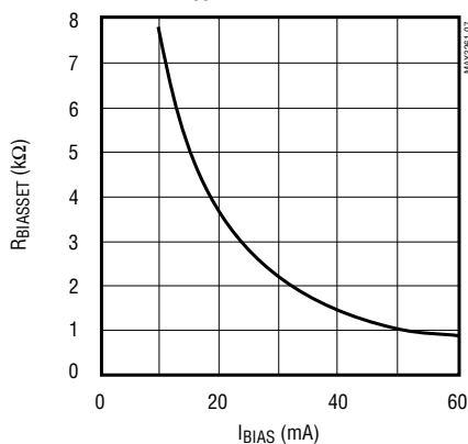
RBIASSET VS. BIAS CURRENT
