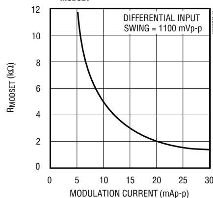
RMODSET VS. MODULATION CURRENT
