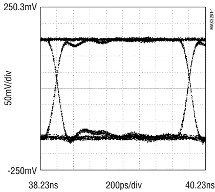
EYE DIAGRAM (622Mbps, LOAD = 25Ω, NOT FILTERED)
