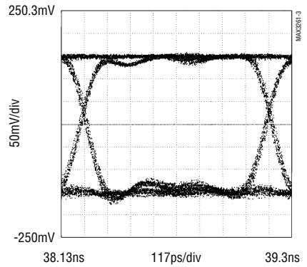
EYE DIAGRAM (1062Mbps, LOAD = 25Ω, NOT FILTERED)
