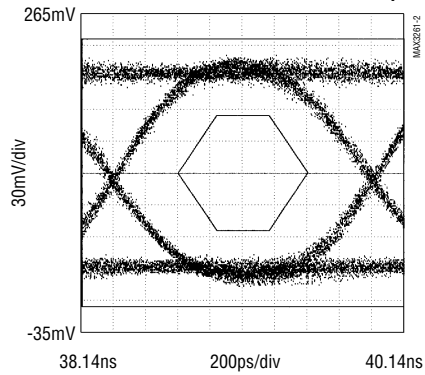
EYE DIAGRAM (622Mbps, LOAD AT OUT- = 1300nm LASER WITH 467MHz BESSEL FILTER)*
