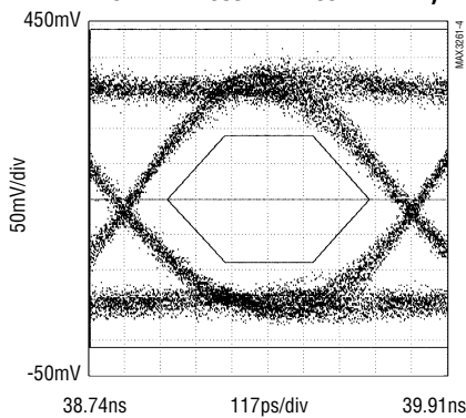
EYE DIAGRAM (1062Mbps, LOAD AT OUT- = 1300nm LASER WITH 800MHz BESSEL FILTER)*
