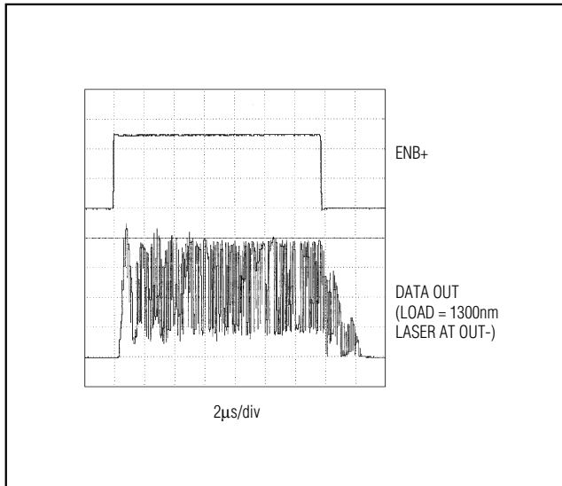
Figure 3. Enable/Disable Operation
