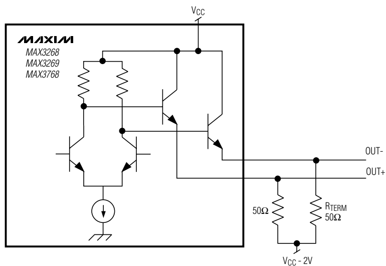
(c) MAX3268/MAX3269/MAX3768 OUTPUT TERMINATION
