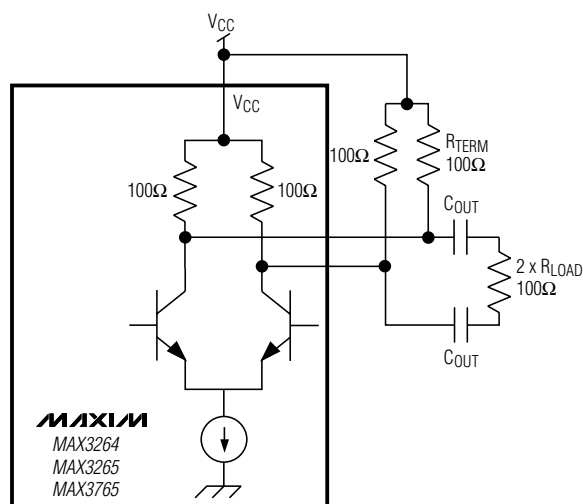
(a) MAX3264/MAX3265/MAX3765 WITH 50Ω TERMINATION
