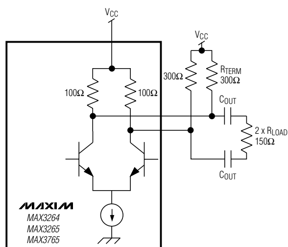
(b) MAX3264/MAX3265/MAX3765 WITH 75Ω TERMINATION
