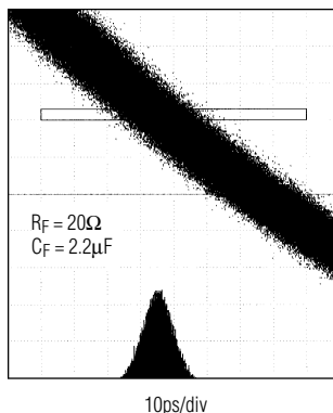
RECOVERED CLOCK JITTER (155Mbps, 1-0 PATTERN, 4.7ps RMS)
