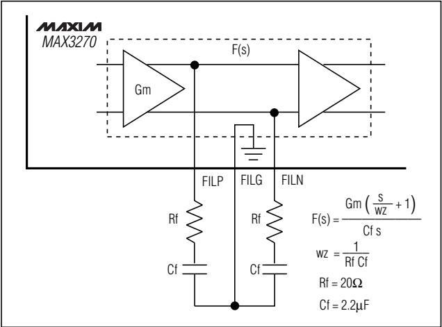
Figure 2. Loop Filter
