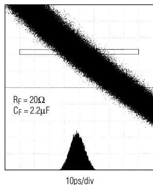
RECOVERED CLOCK JITTER (155Mbps, 2 7 -1 PRBS, 5.1ps RMS)
