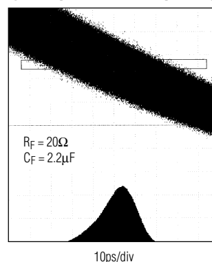
RECOVERED CLOCK JITTER (622Mbps 2 7 -1 PRBS 9.0ps RMS)
