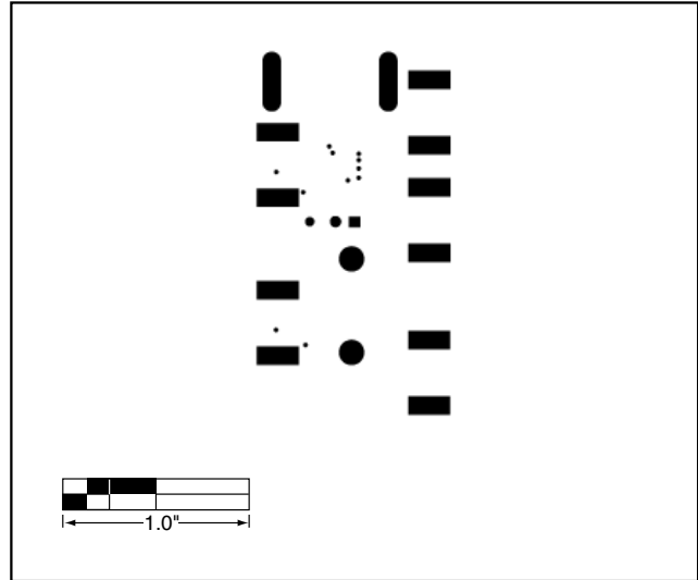
Figure 6. MAX3271 EV Kit PC Board Layout—Solder Side
