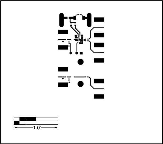
Figure 3. MAX3271 EV Kit PC Board Layout—Component Side
