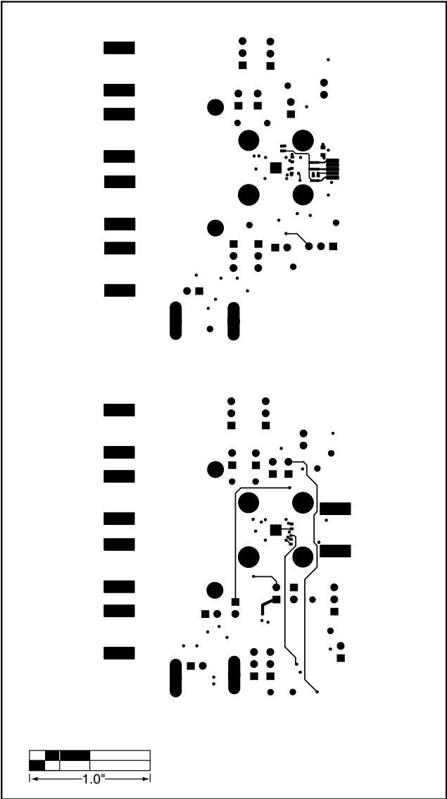
Figure 8. MAX3273 EV Kit PC Board Layout—Solder Side
