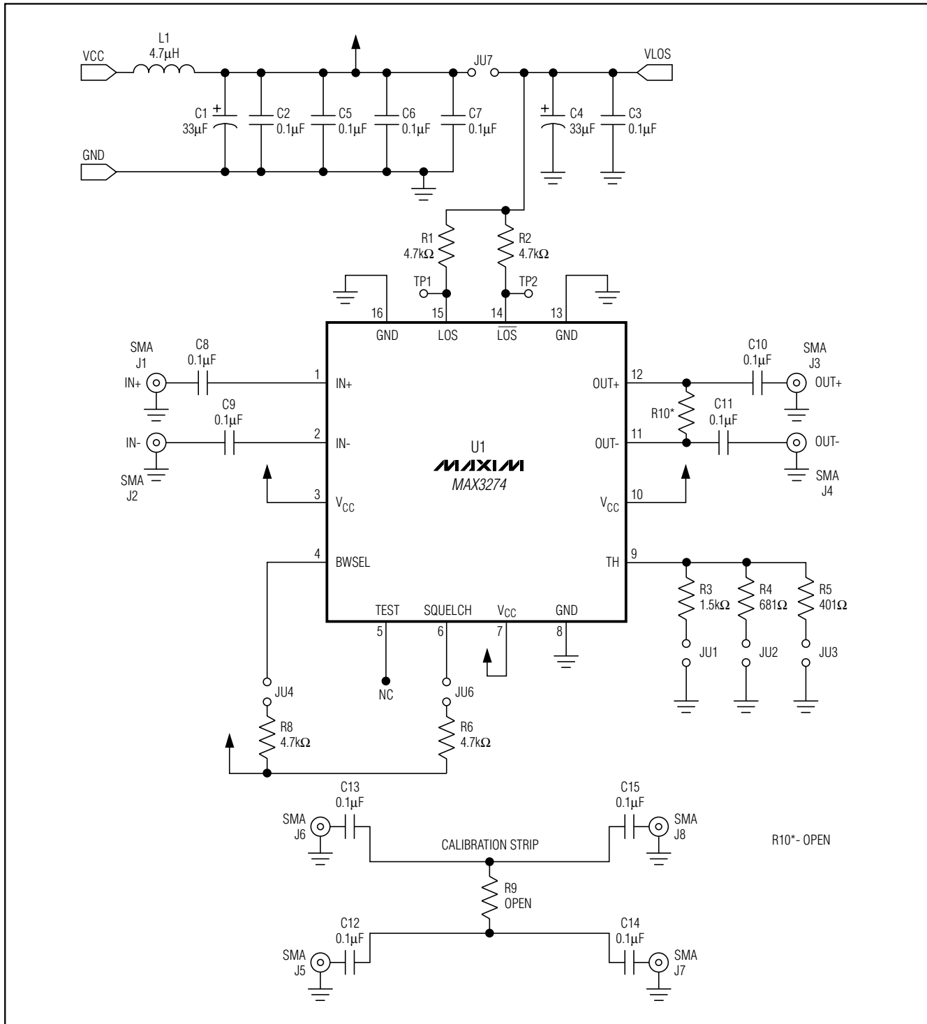
Figure 1. MAX3274 EV Kit Schematic
