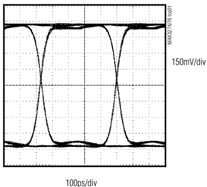
INPUT = 1.2V p-p , 2 7 - 1 PRBS, BWSEL = 1
