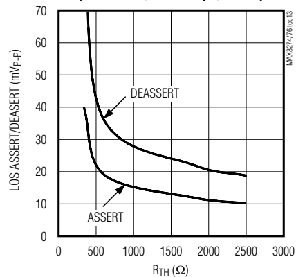
ASSERT/DEASSERT LEVELS vs. R_{TH} (BWSEL = 1, 2.125Gbps, K28.5)
