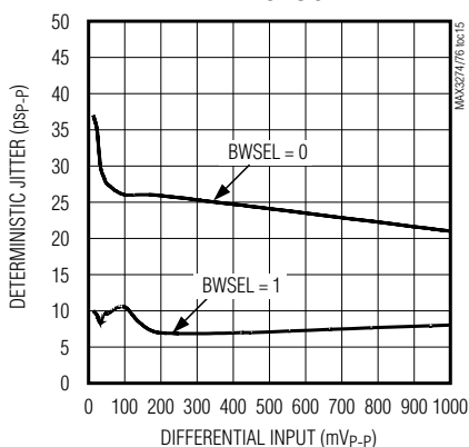
DETERMINISTIC JITTER
