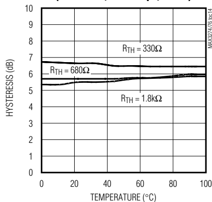
LOS HYSTERESIS vs. TEMPERATURE (BWSEL = 1, 2.125Gbps, K28.5)
