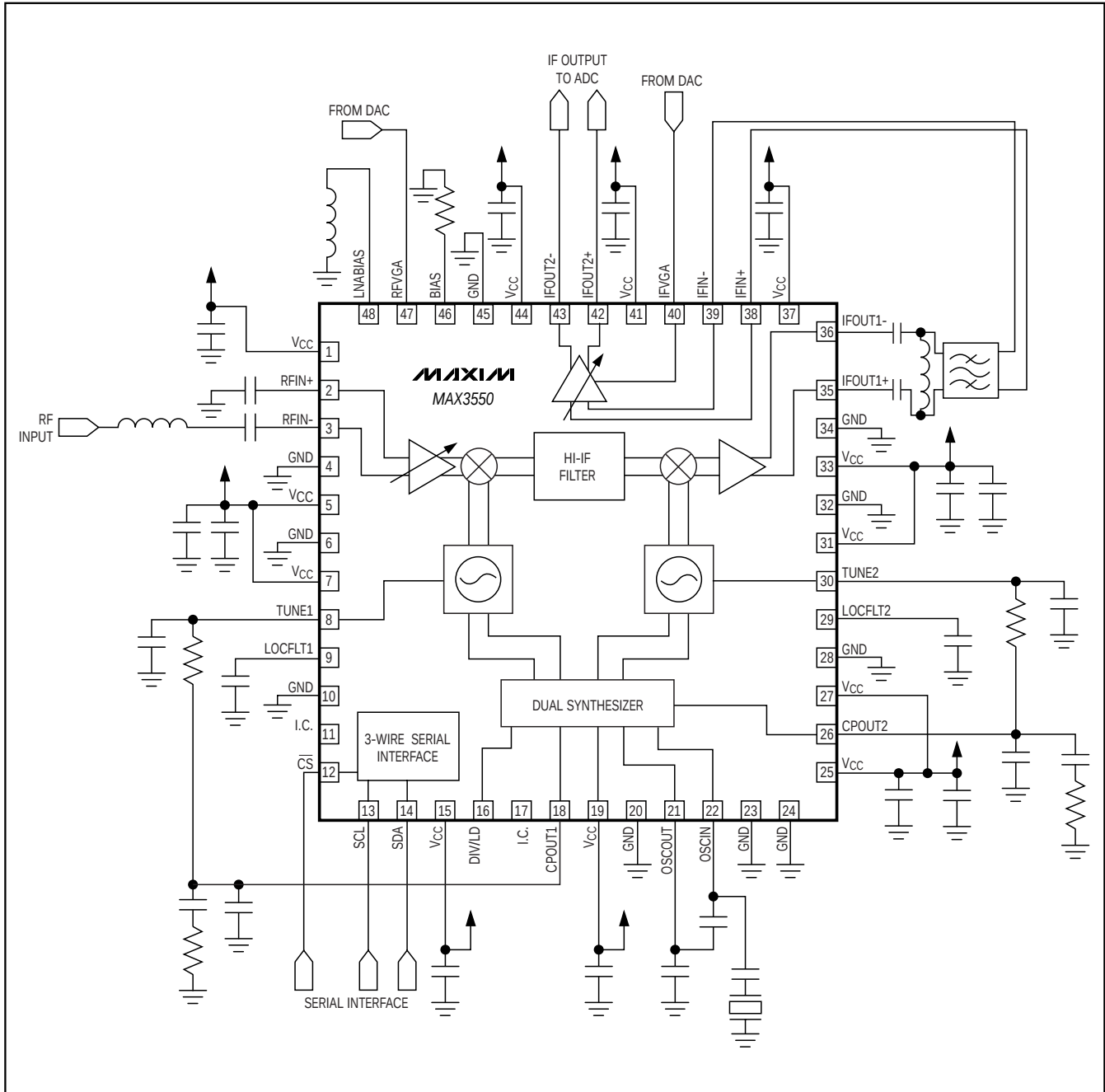
Typical Application Circuit
