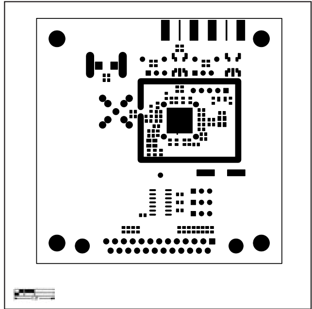
Figure 4. MAX355x Evaluation Kit PC Board Layout—Top Soldermask
