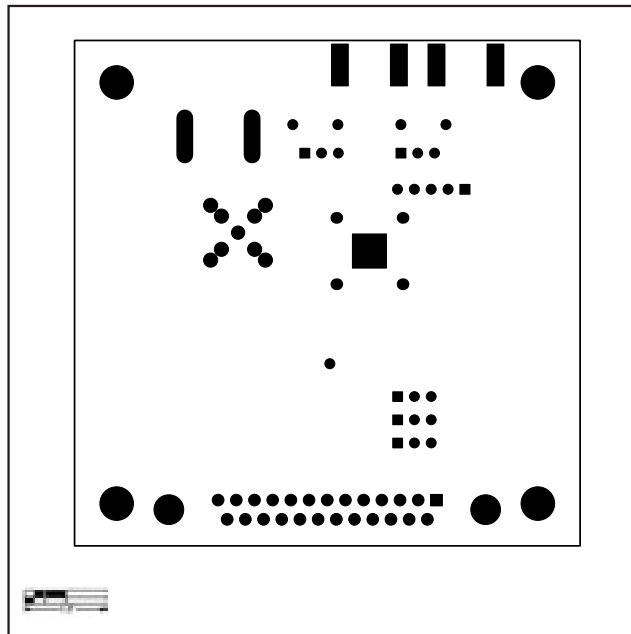
Figure 9. MAX355X_EV Kit PC Board Layout—Bottom Soldermask
