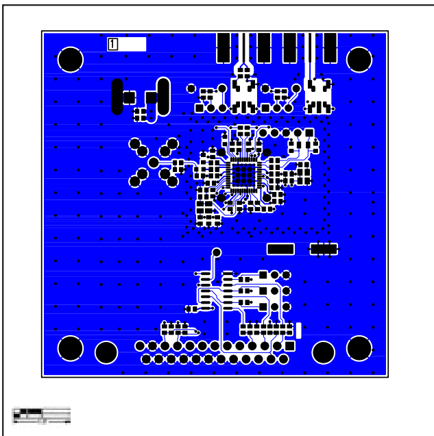
Figure 5. MAX355x Evaluation Kit PC Board Layout—Primary Component Side
