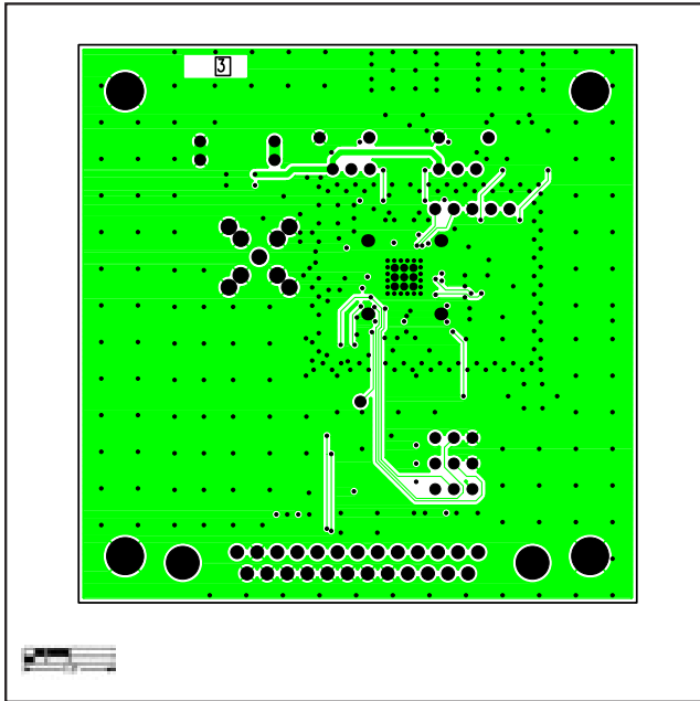
Figure 7. MAX355X_EV Kit PC Board Layout—Inner Layer 3
