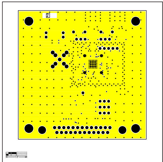
Figure 6. MAX355x Evaluation Kit PC Board Layout—Inner Layer 2
