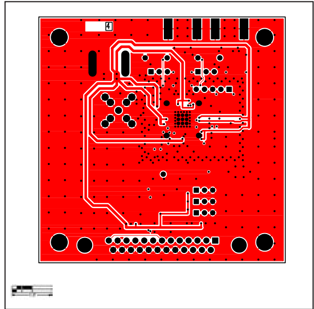
Figure 8. MAX355X_EV Kit PC Board Layout—Secondary Component Side
