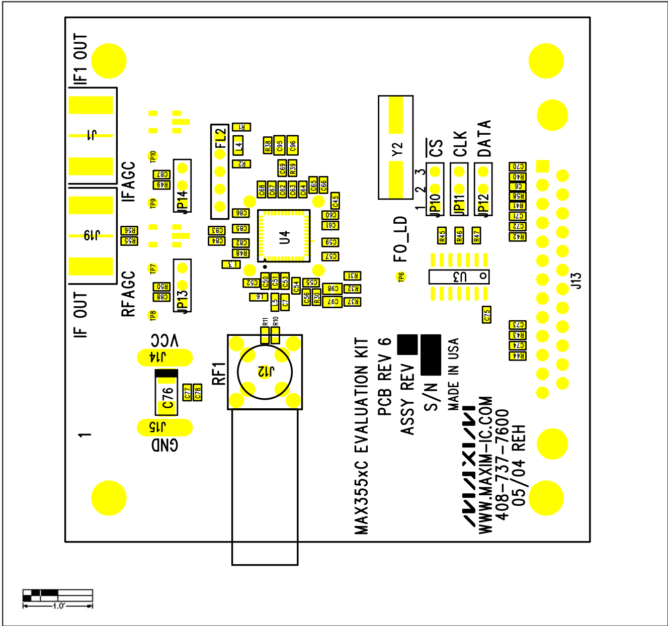
Figure 2. MAX355_ EV PC Board Layout—Component Placement Guide
