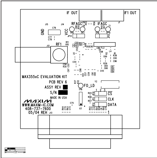
Figure 3. MAX355x Evaluation Kit PC Board Layout—Top Silkscreen
