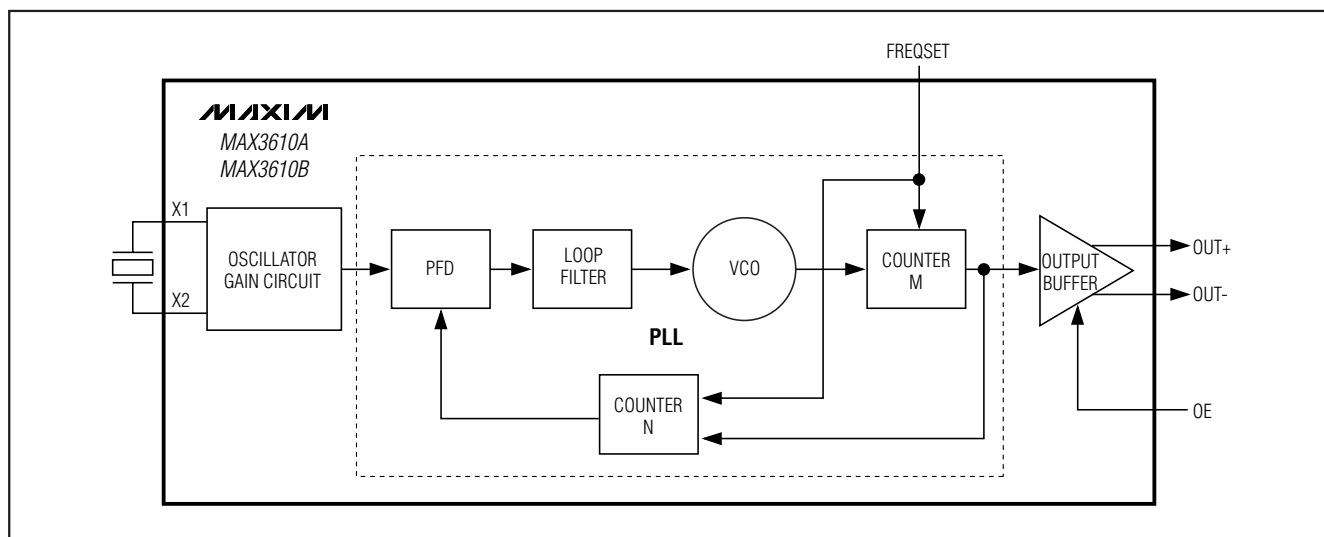
Figure 2. Functional Diagram
