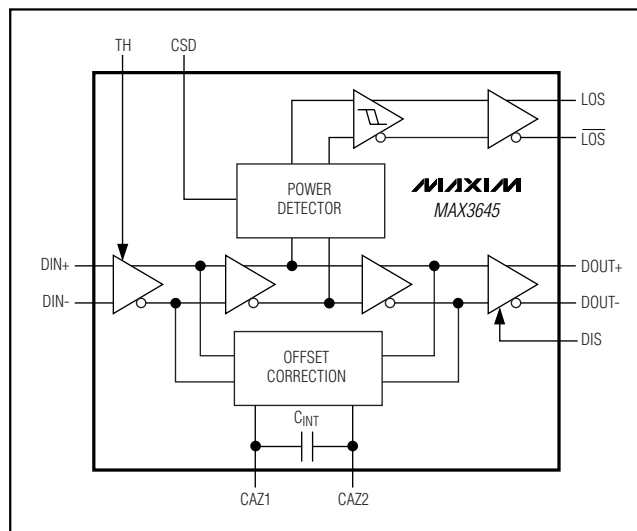
Figure 2. Functional Diagram
