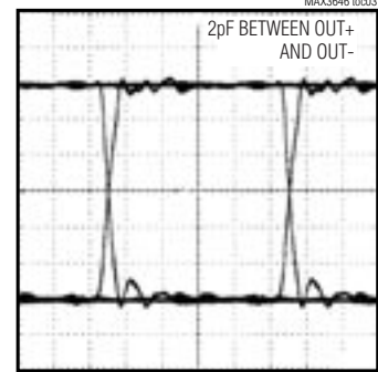
ELECTRICAL EYE DIAGRAM ( I_{MOD} = 30mA , 622.08MHz, 2^7 - 1 PRBS)
