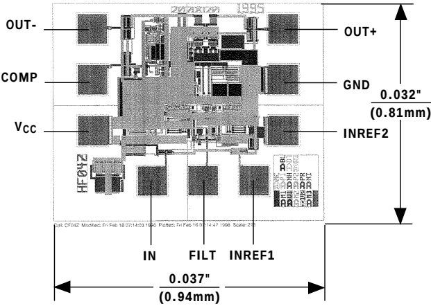
Chip Topography
