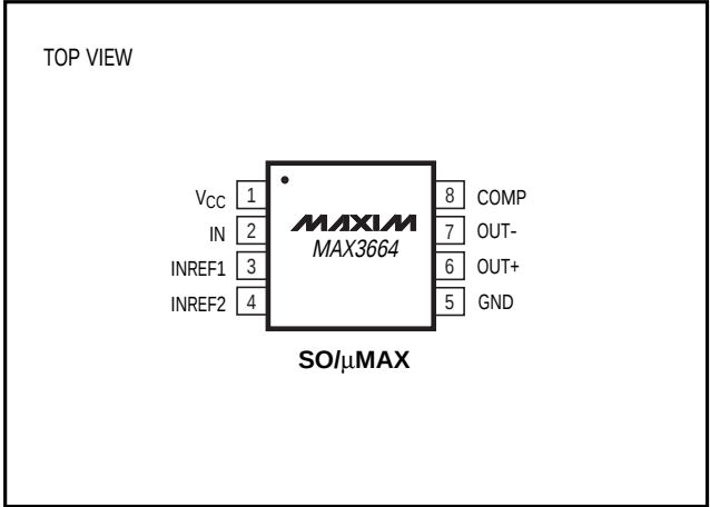
Pin Configuration
