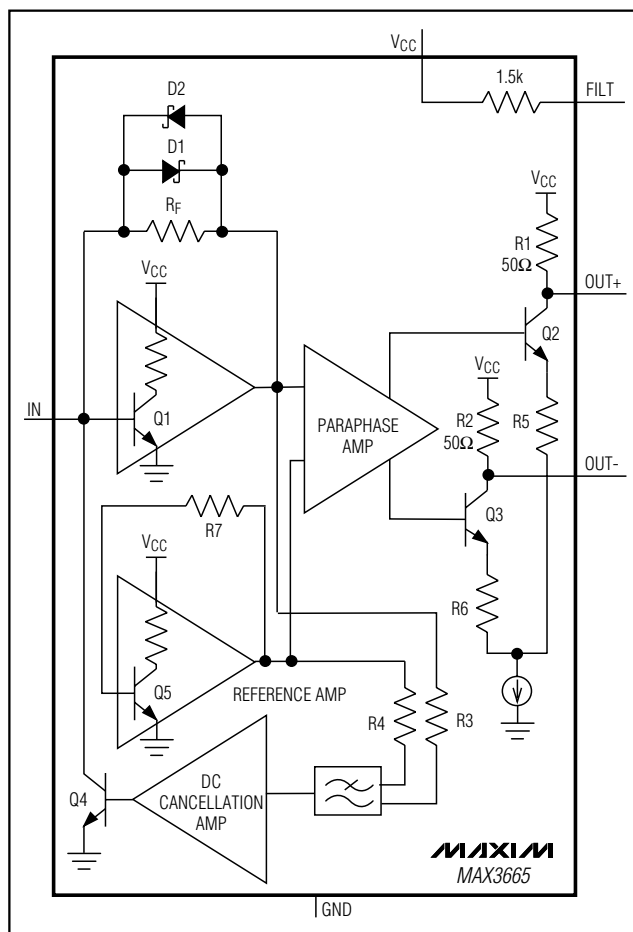
Figure 1. Functional Diagram
