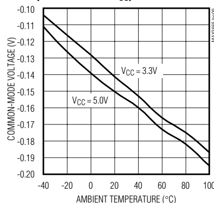
OUTPUT COMMON-MODE VOLTAGE (REFERENCED TO V_{CC} ) vs. TEMPERATURE
