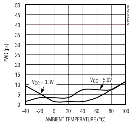
PULSE-WIDTH DISTORTION vs. TEMPERATURE (INPUT = 450 \mu A-p)
