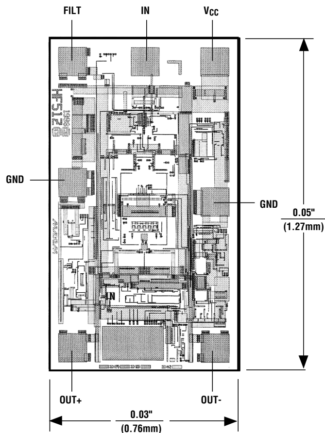
Chip Topography
