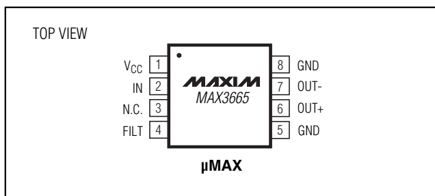
Pin Configuration
