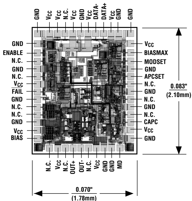
Chip Topography
