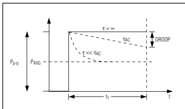
Figure 4. Droop
