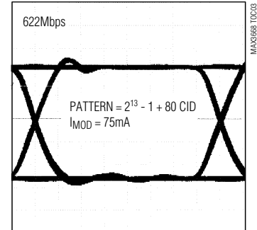
EYE DIAGRAM ( I_{MOD} = 75mA )
