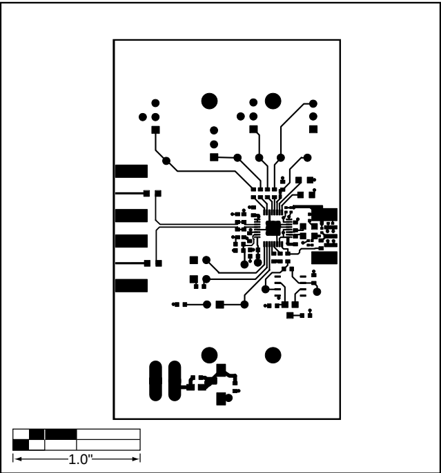
Figure 5. MAX3669 EV Kit PC Board Layout—Component Side
