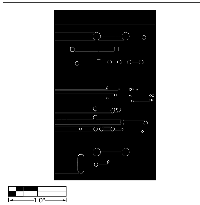
Figure 7. MAX3669 EV Kit PC Board Layout—Ground Plane
