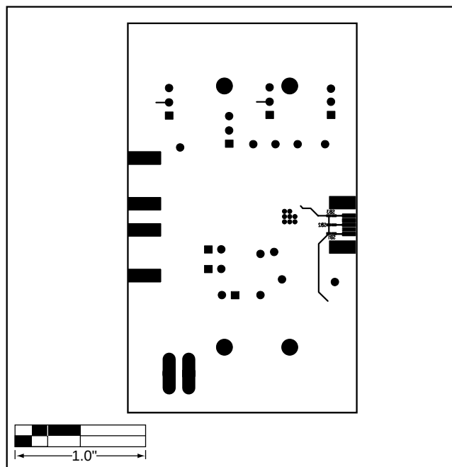
Figure 9. MAX3669 EV Kit Component Placement Guide—Solder Side
