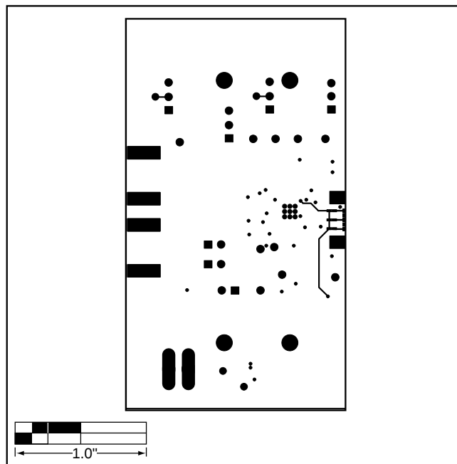
Figure 6. MAX3669 EV Kit PC Board Layout—Solder Side
