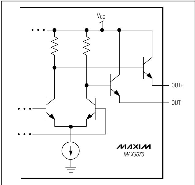
Figure 2. Output Interface
