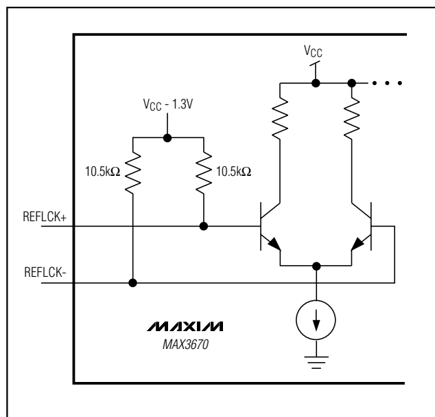
Figure 1. Input Interface
