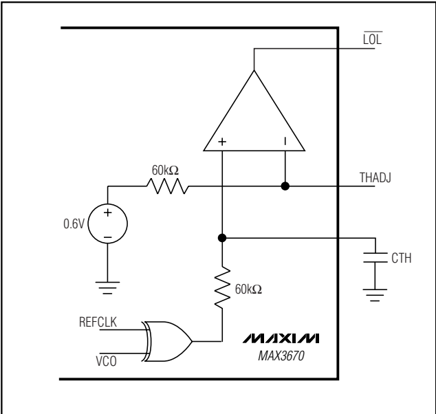
Figure 3. Loss-of-Lock Indicator
