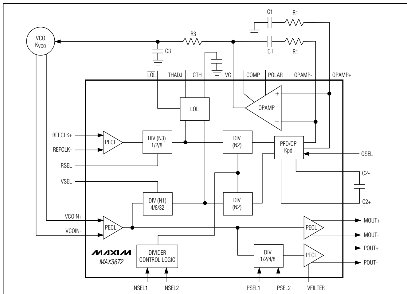
Functional Diagram
