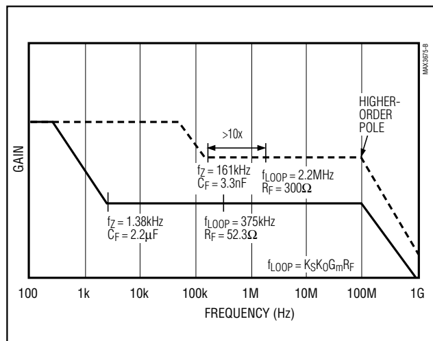
Figure 3. Loop-Filter Response
