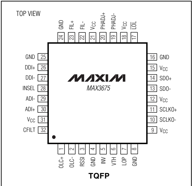
Pin Configuration
