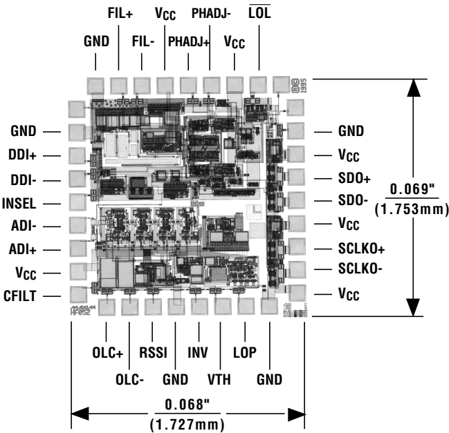
Chip Topography
