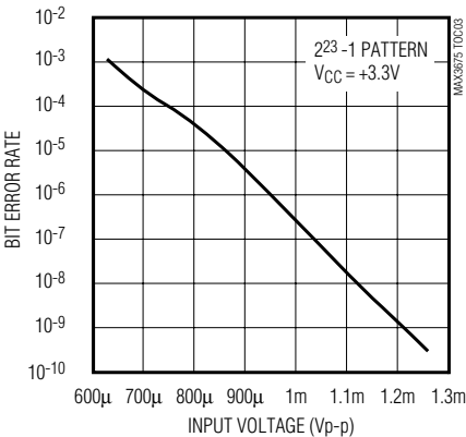
BIT ERROR RATE vs. INPUT VOLTAGE
